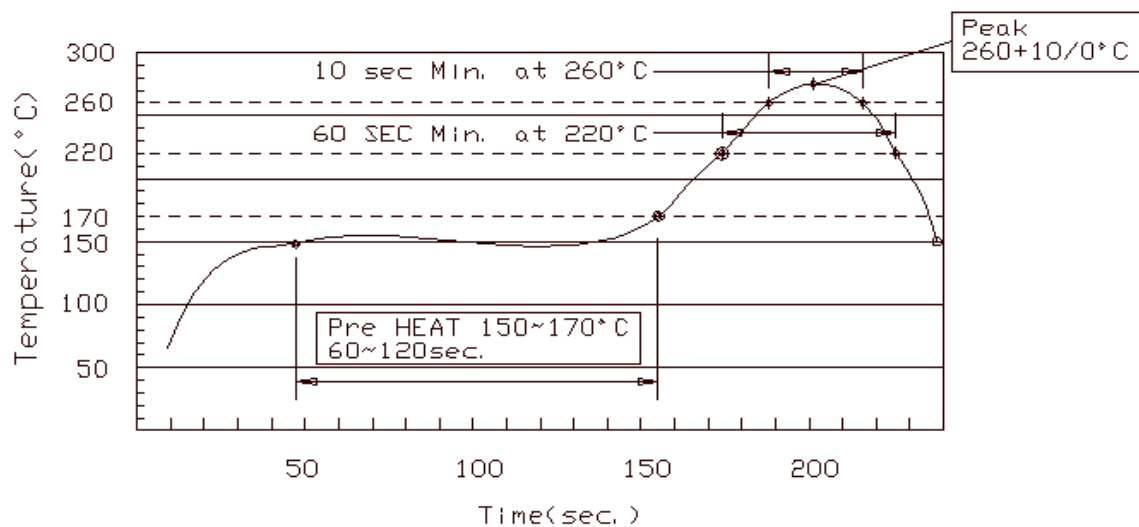
Fig.1 Temperature profile of Infrared Reflow Soldering for evaluation
